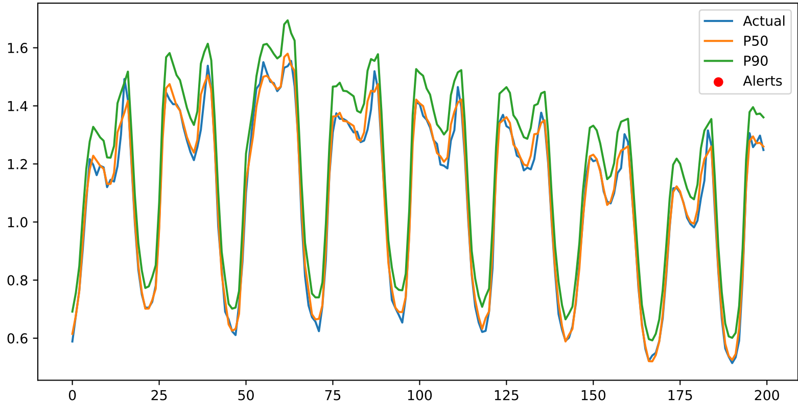
Operational Peak Demand Alerts using P90 Forecasts
